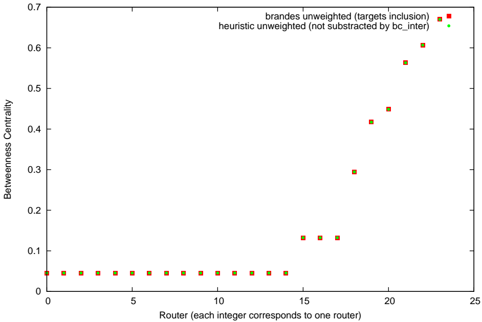
Centrality for jsoninfo_topo_unweighted
